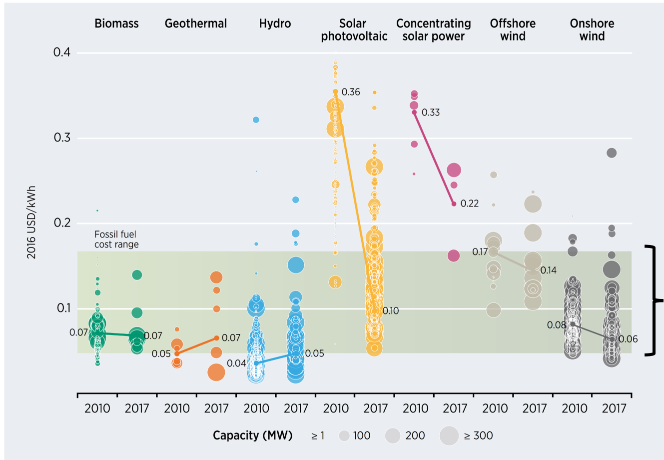
Figure 2.1 Global levelised cost of electricity from utility-scale renewable power generation technologies, 2010-2017
